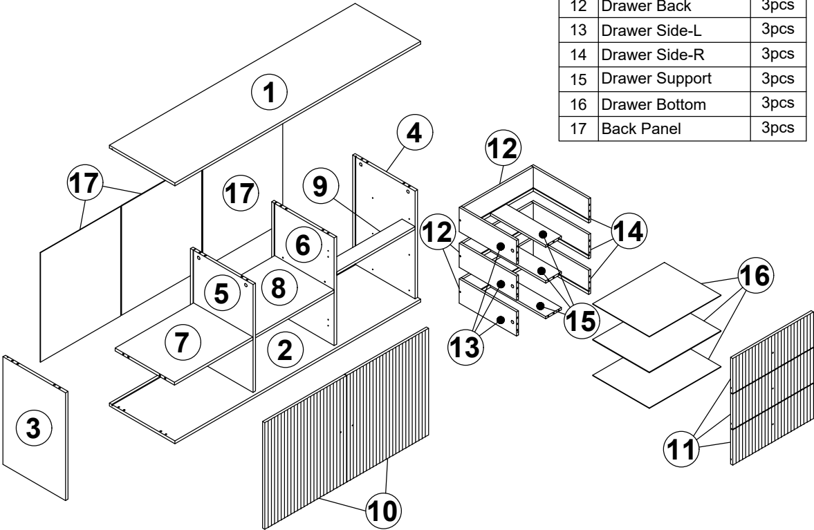
COMPLETE ASSEMBLY
