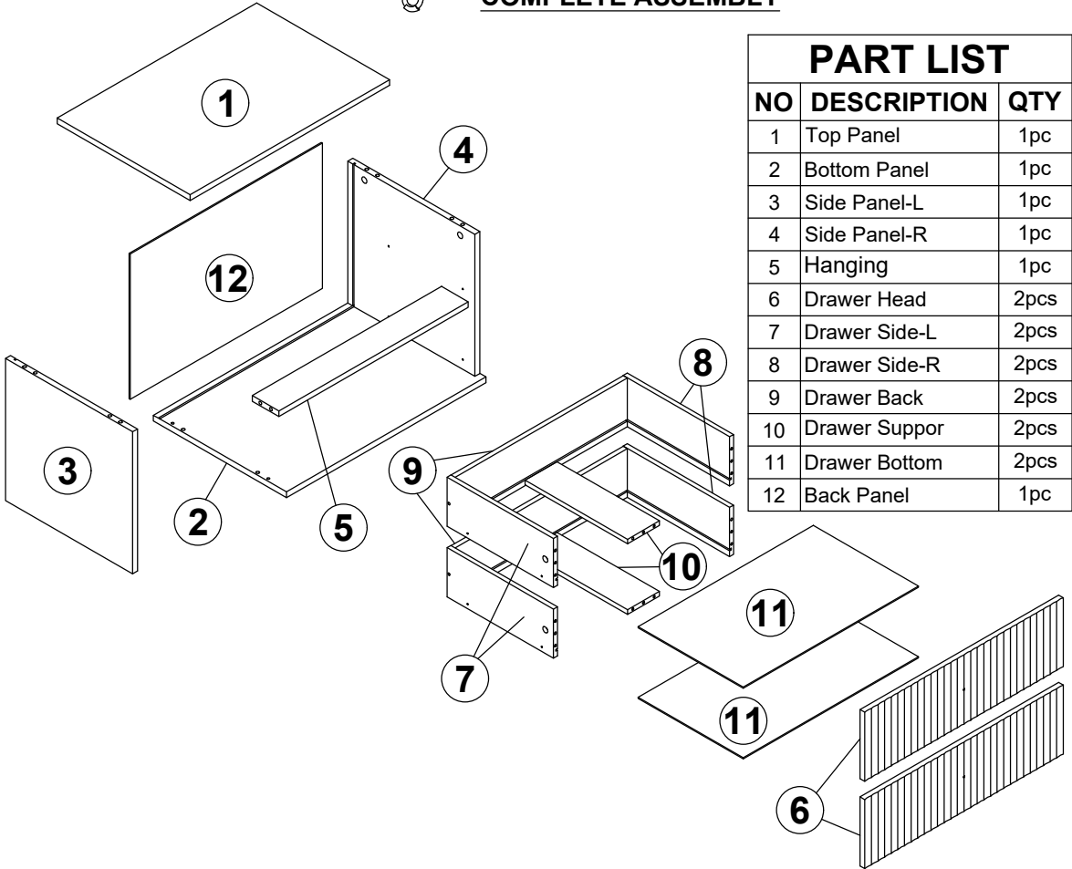
COMPLETE ASSEMBLY
