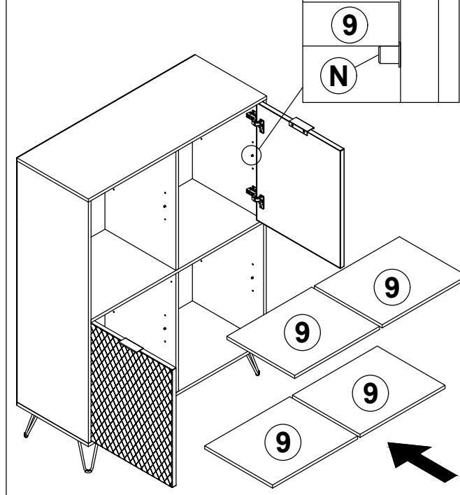
Step 17
