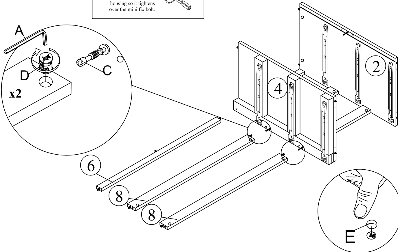
*Attach Minifix Cap as shown.
