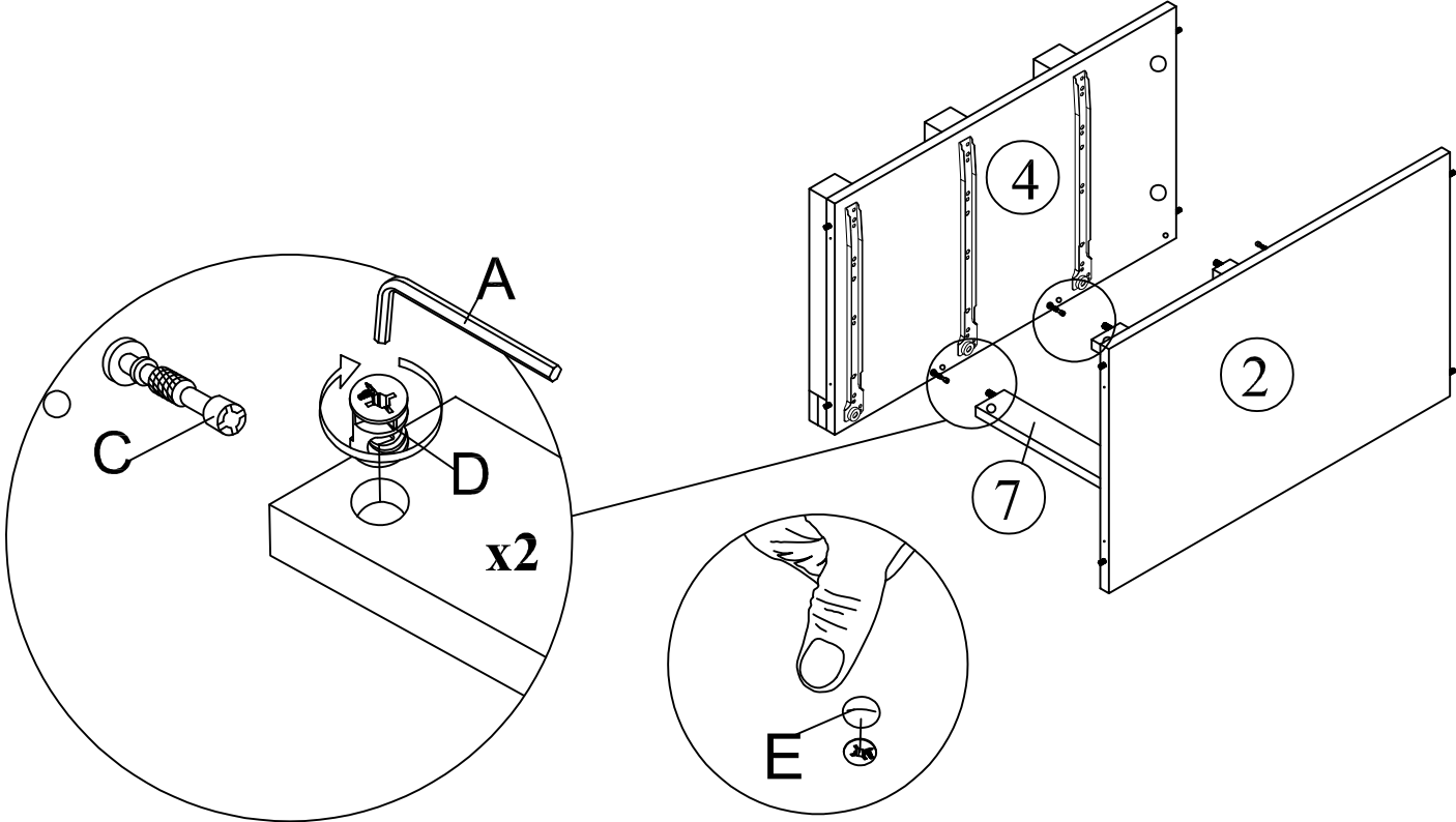
*Attach Minifix Cap as shown.
